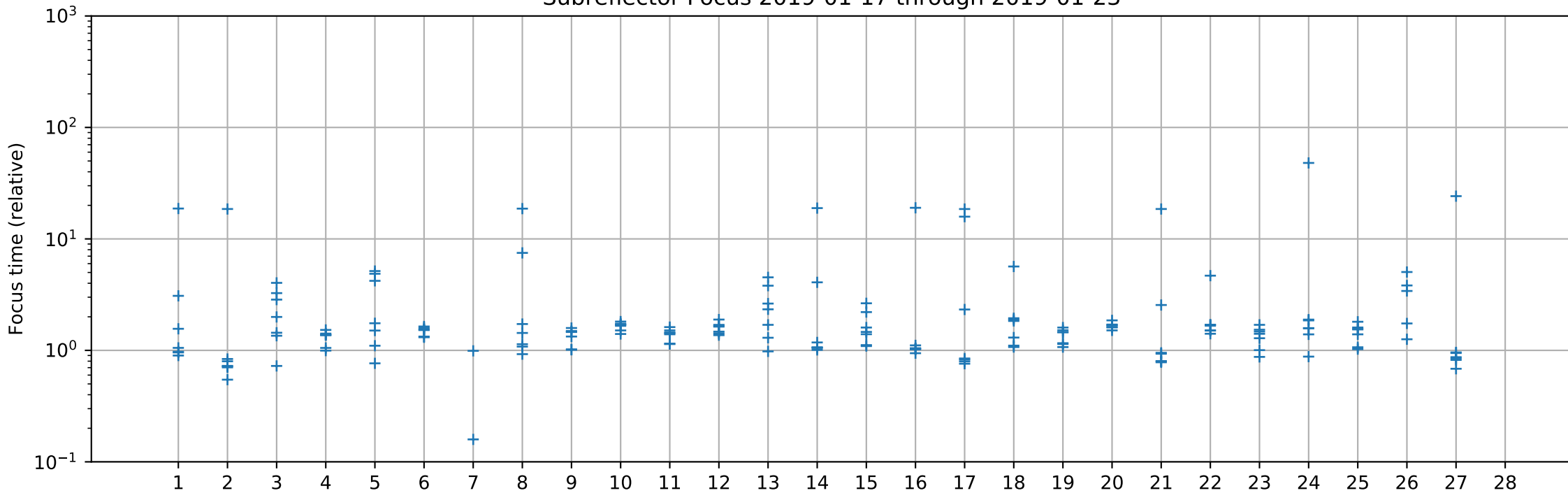
Subreflector Focus 2019-01-17 through 2019-01-23
