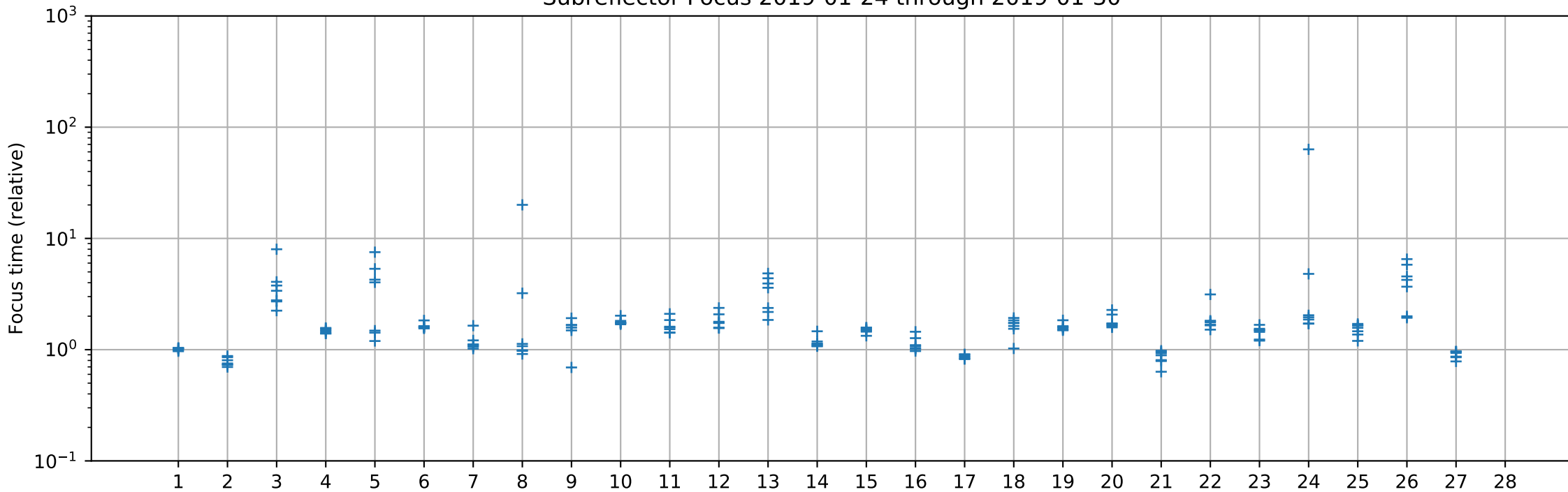
Subreflector Focus 2019-01-24 through 2019-01-30
