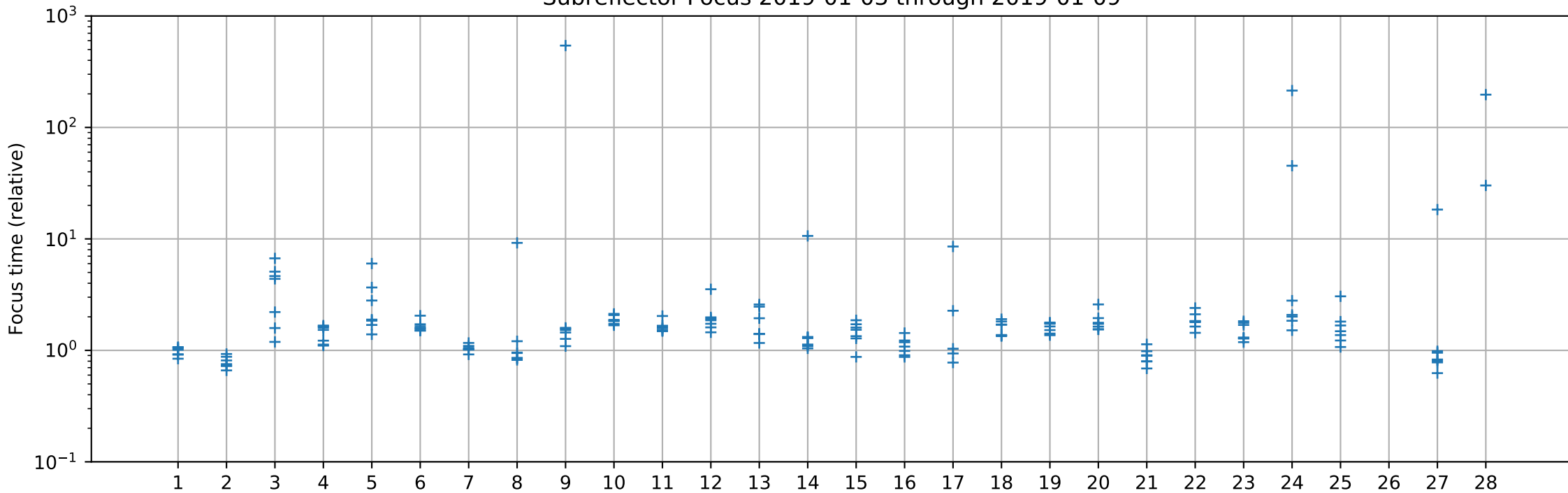
Subreflector Focus 2019-01-03 through 2019-01-09
