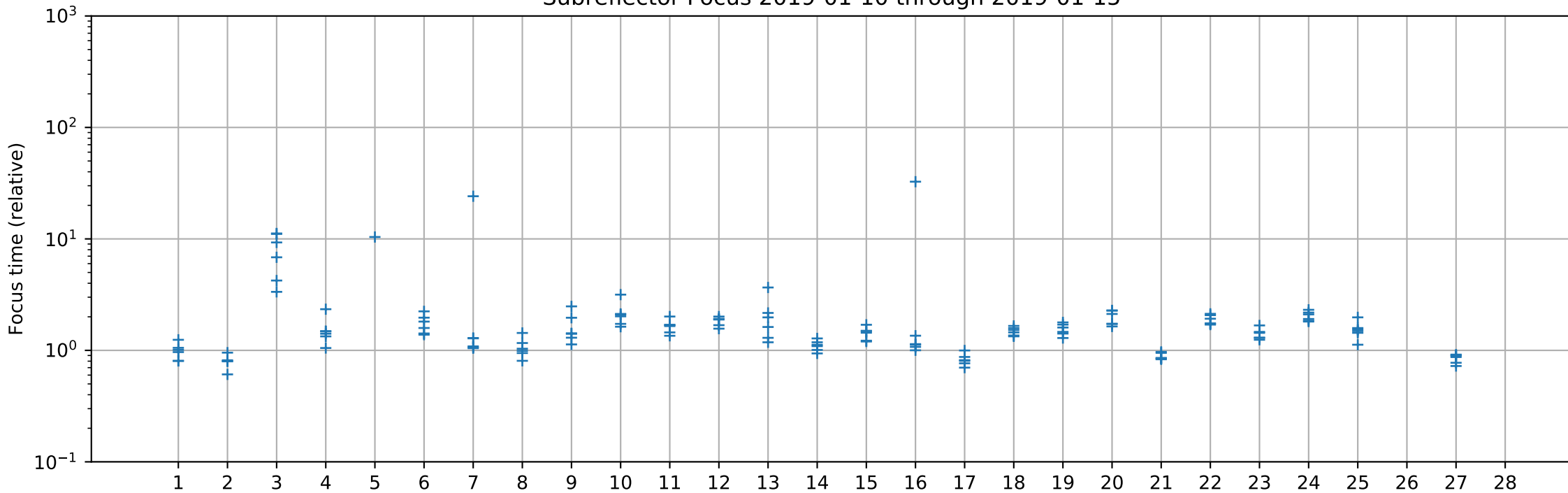
Subreflector Focus 2019-01-10 through 2019-01-15
