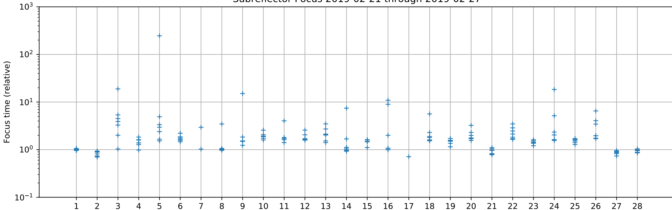
Subreflector Focus 2019-02-21 through 2019-02-27
