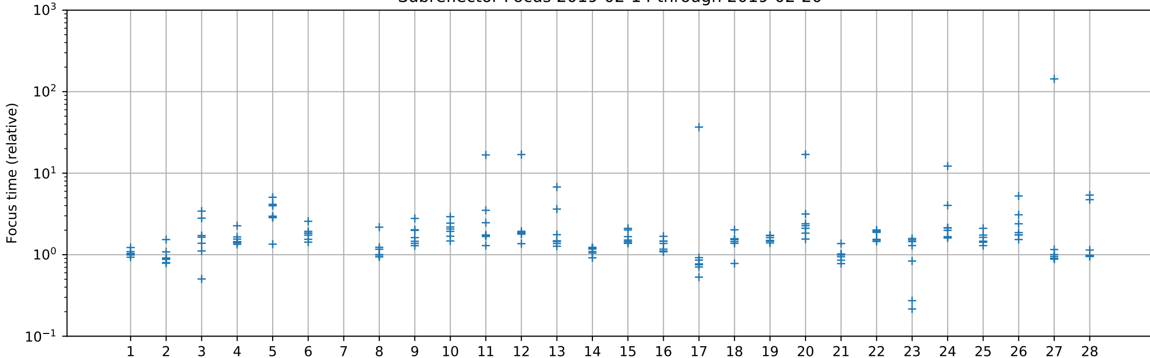
Subreflector Focus 2019-02-14 through 2019-02-20
