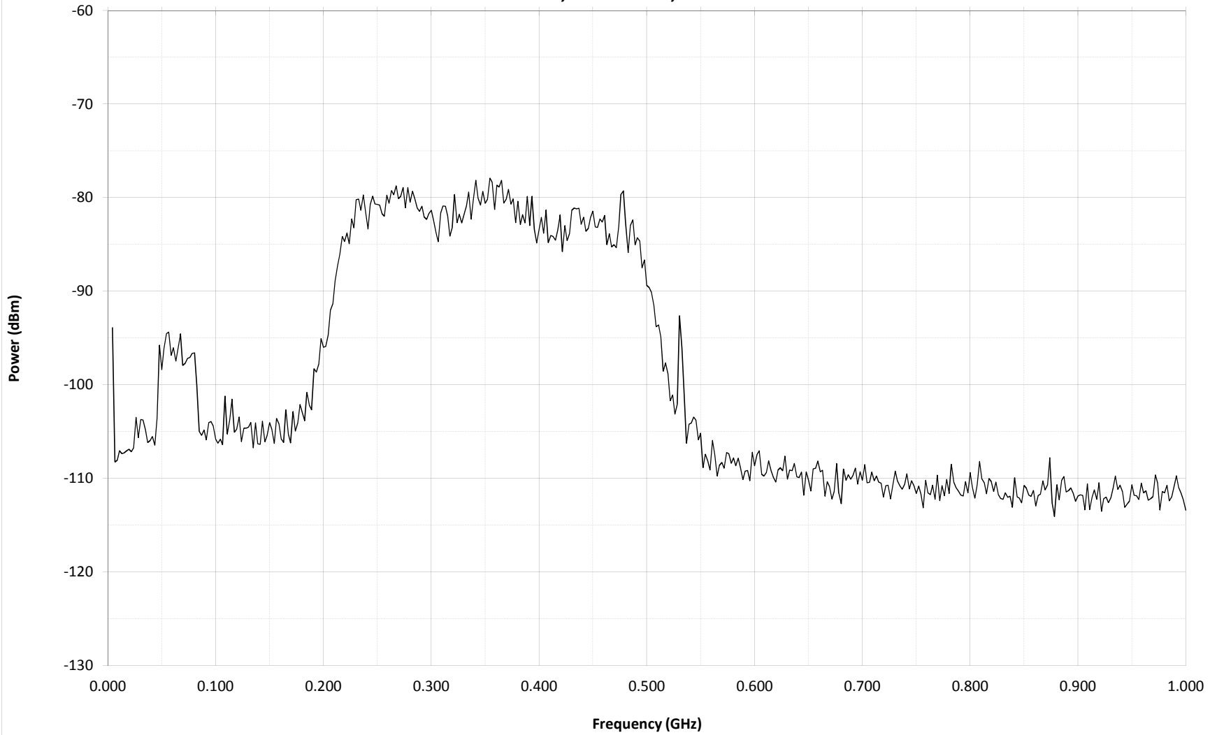
File: ea23VR2.CSV = ea23 R/Y/H side @ Vertex Room, LOIF rack input 20150320, 15:00 MDT, 100 KHz RBW
