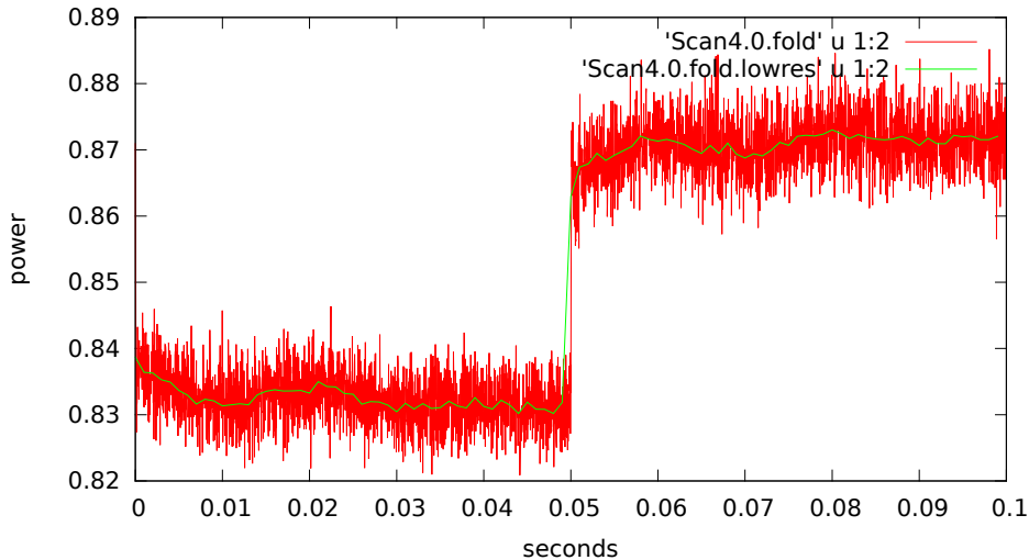
Summed-array folded switched power
