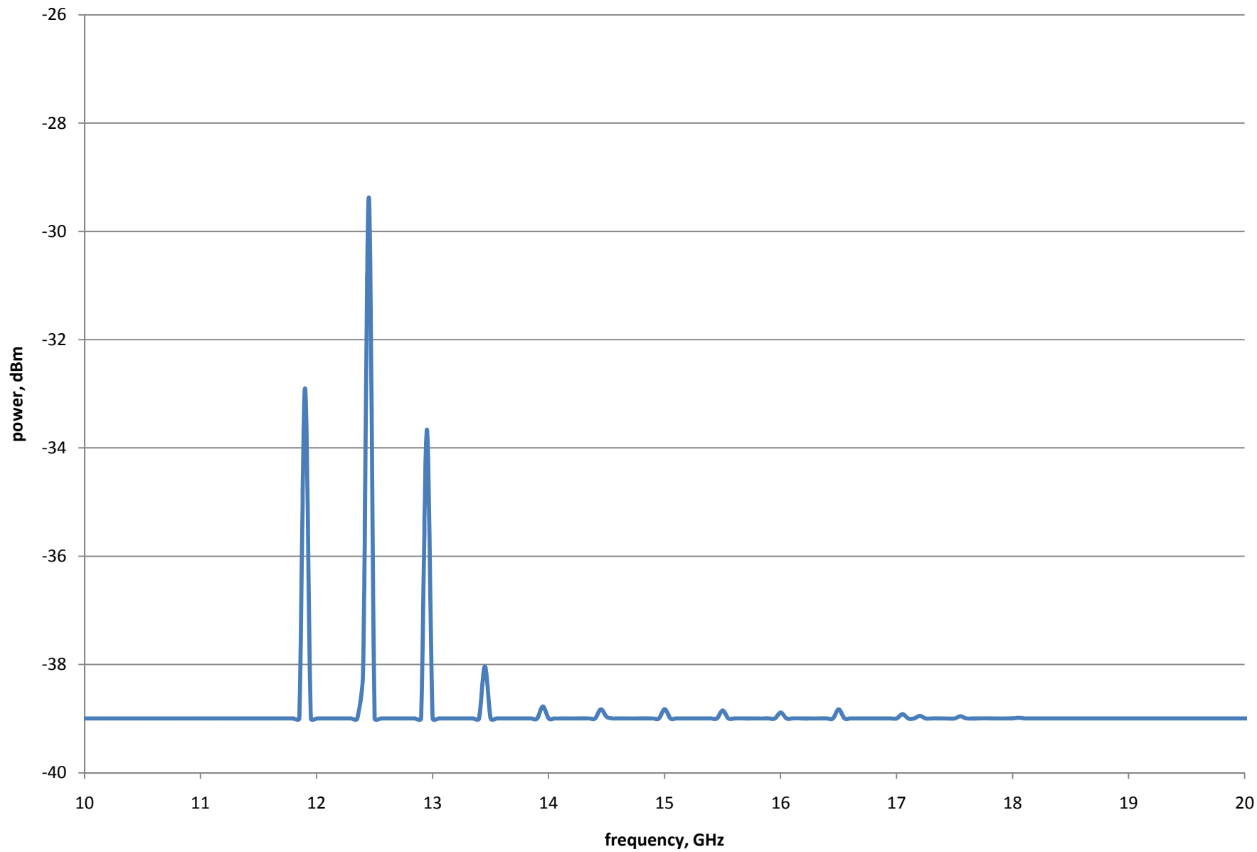
T302 filtered LO leakage on nominal T304 input noise power
