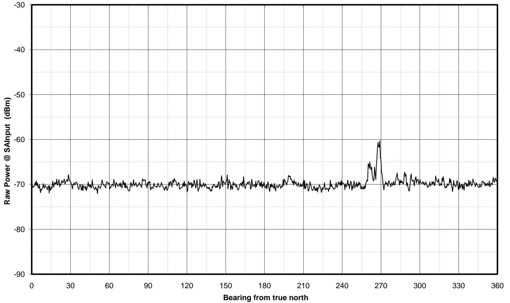
RF-DFS power levels vs. bearing at: 6 GHz
